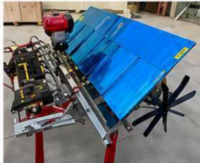
PADDY TRANSPLANTER
